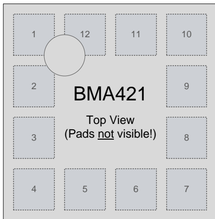
Pin configuration (top view)
