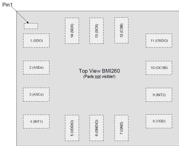
Pin-out top view
