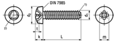
1) Tapered thread end max. 4P 2) Trilobular
