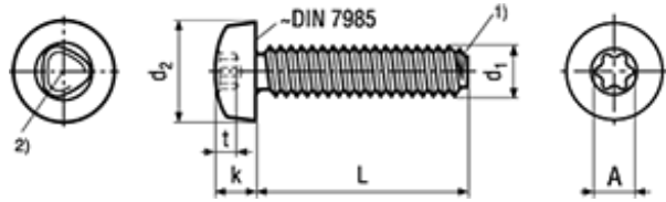
1) Tapered thread end max. 4P 2) Trilobular
