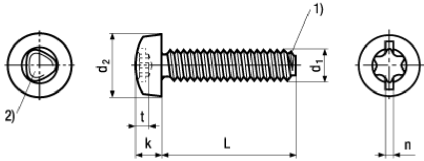
1) Tapered thread end max. 4P 2) Trilobular cross-section
