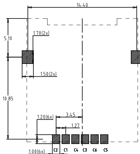
PCB LAYOUT
