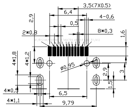
RECOMMENDED P.C.B. LAYOUT TOLERANCE UNSPECIFIED ±0.05mm
