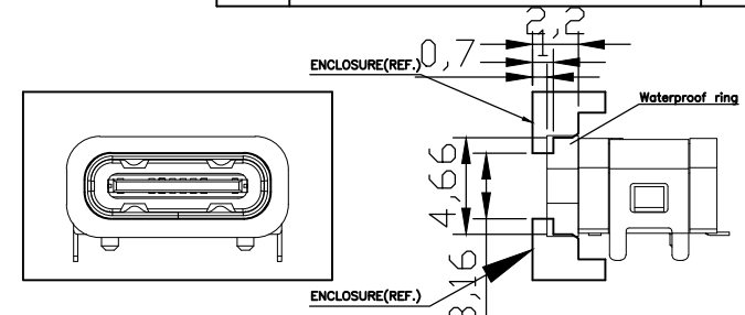
RECOMMENDED SCHEMATIC DRAWING OF CONNECTOR MATCH CHASSIS
