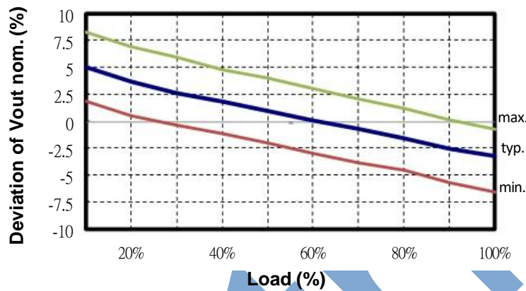
5VDC Output
