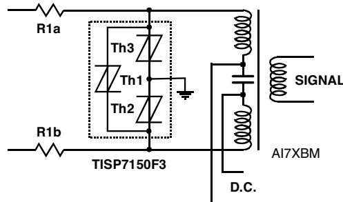
Figure 21. ISDN Protection
