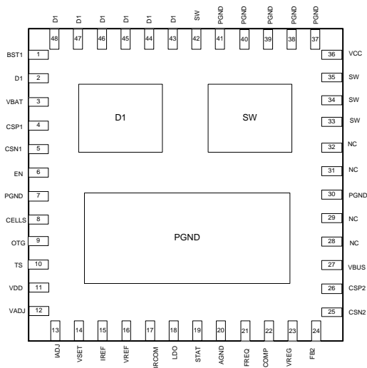
Fig. 3 Pin-Function (QFN6X6-48)
