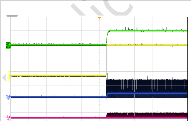
Fig.6 Start up waveform, Iout =0A
