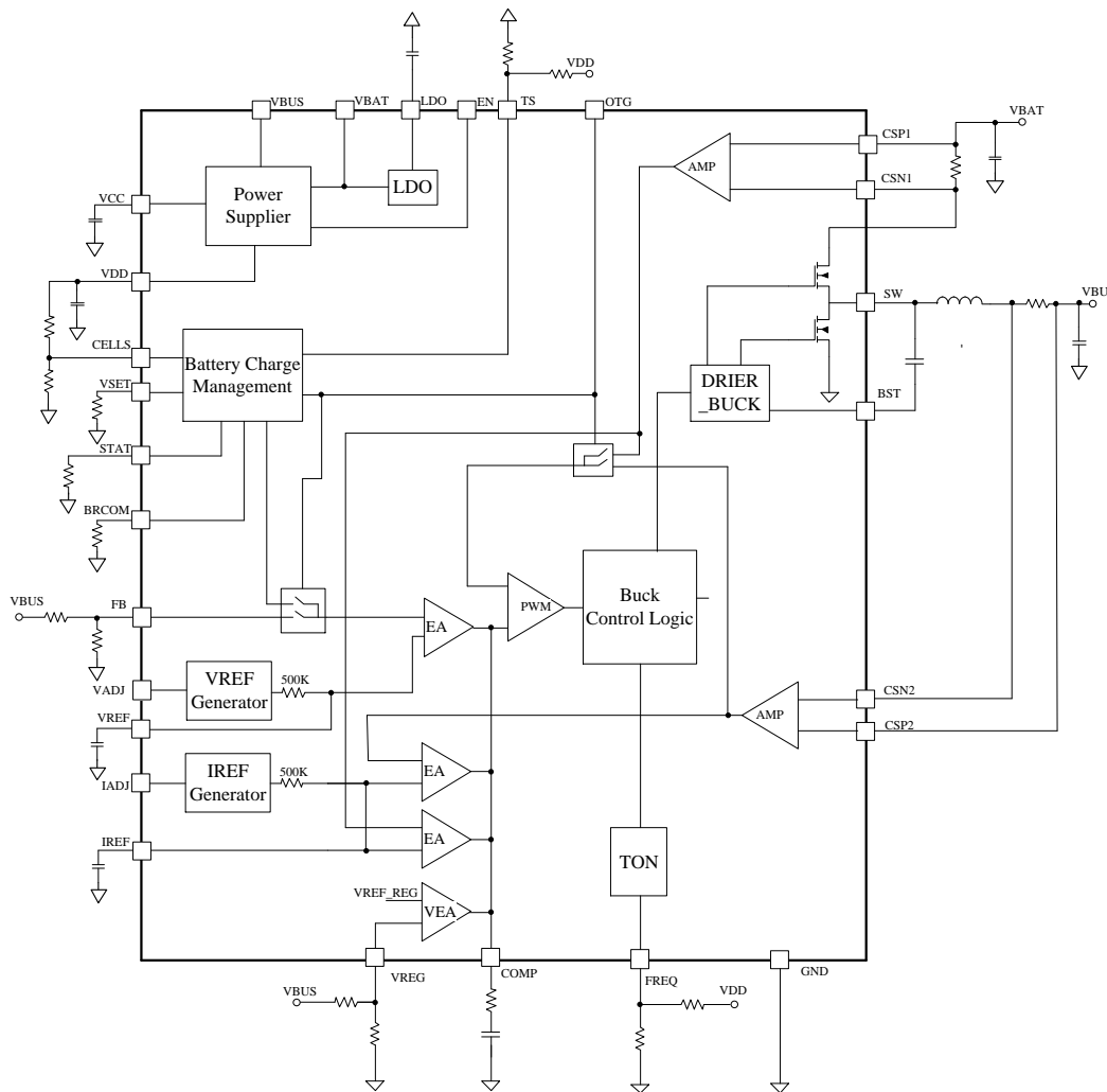
Fig. 22 PL8405 Block Diagram
