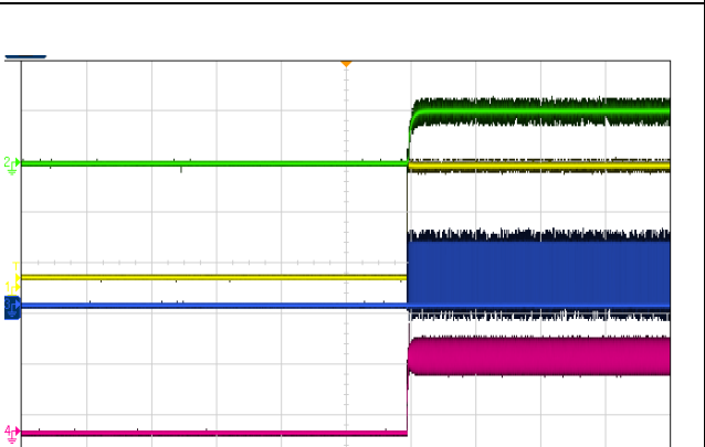
Fig.7 Start up waveform, Iout =5A
