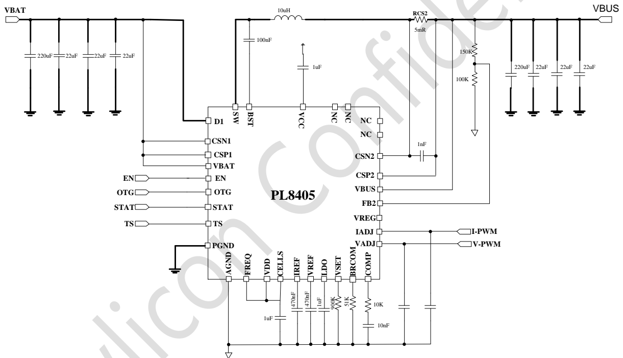
Fig. 23 Application Schematic (VBAT:24V VBUS:5V IOU:5A)
