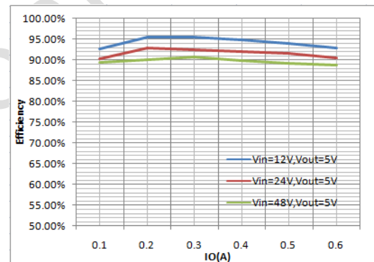
Fig. 2 Efficiency
