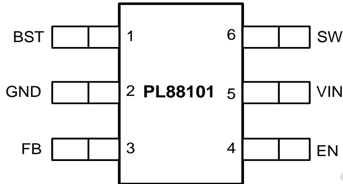
Fig.3 SOT23-6L Package
