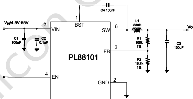
Fig 24 Schematic
