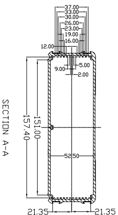
ENCLOSURE PROFILE
