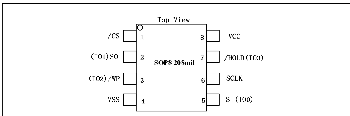
Figure 2. Pin Configuration SOP 150mil/208 mil
