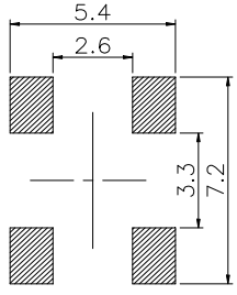
PCB. 焊接图 PCB. WELDING DRAWING
