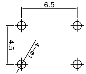
PCB. 焊接图 PCB. WELDING DRAWING
