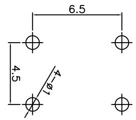
PCB. 焊接图 PCB. WELDING DRAWING
