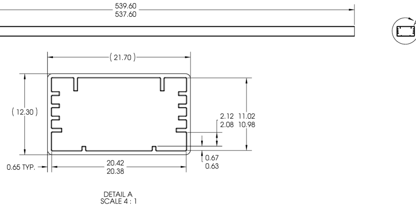
Figure 46: Tube Design for Hexagonal Star Products
