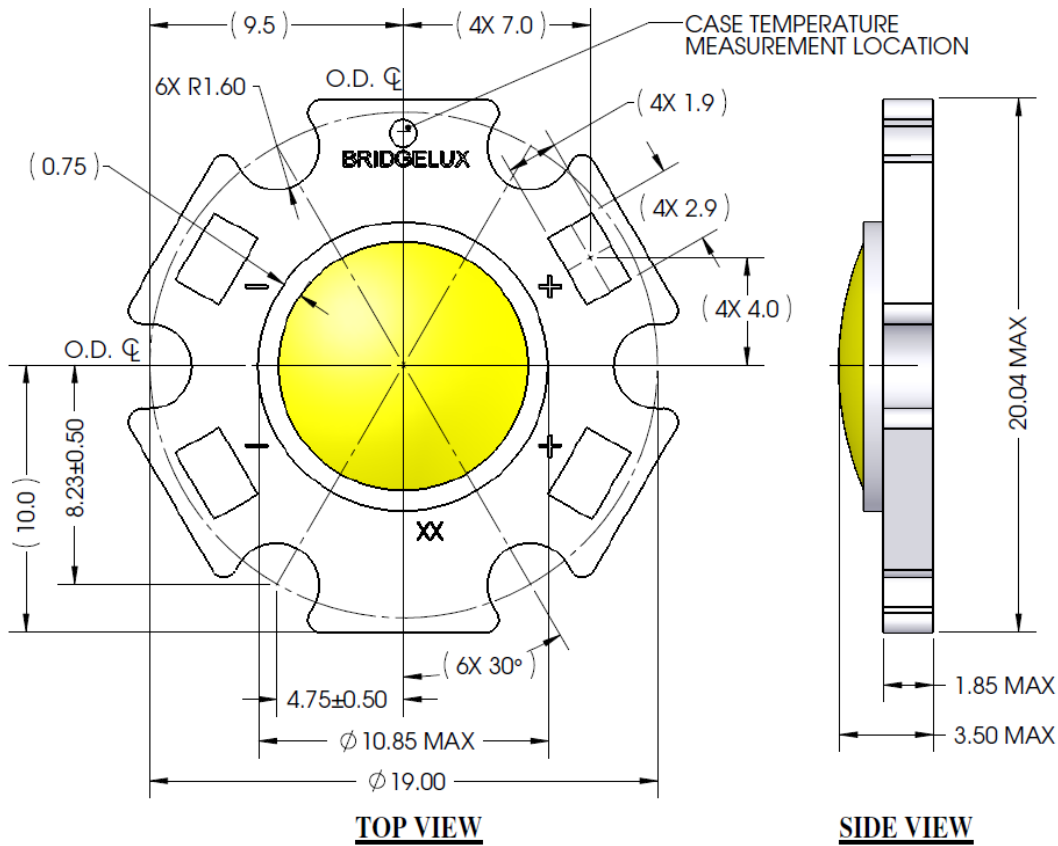
Figure 1: Drawing for 400 lumen product options (part numbers BXRA-C0402, BXRA-N0402, BXRA-W0401, BXRA-W0403, BXRA-W0402 and BXRA-C0603).
