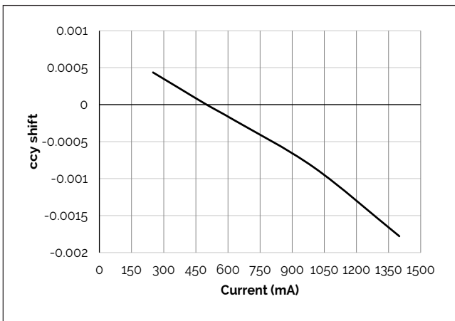
Figure 11: V13C Drive Current vs. ccx Shift
