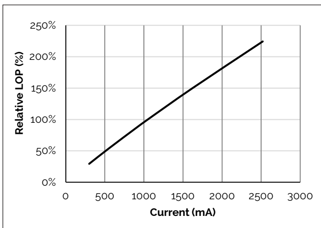
Figure 5: V22C Typical Relative Flux vs. Current
