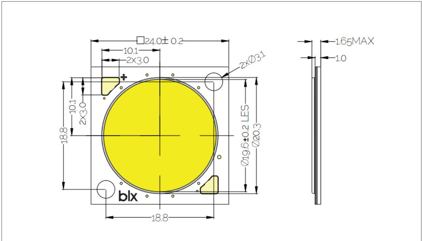
Figure 16: V18 LED Array
