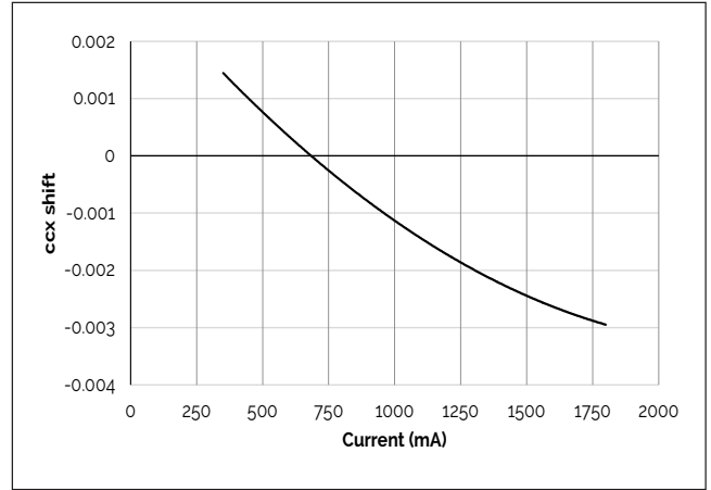
Figure 8: V18B Drive Current vs. ccx Shift
