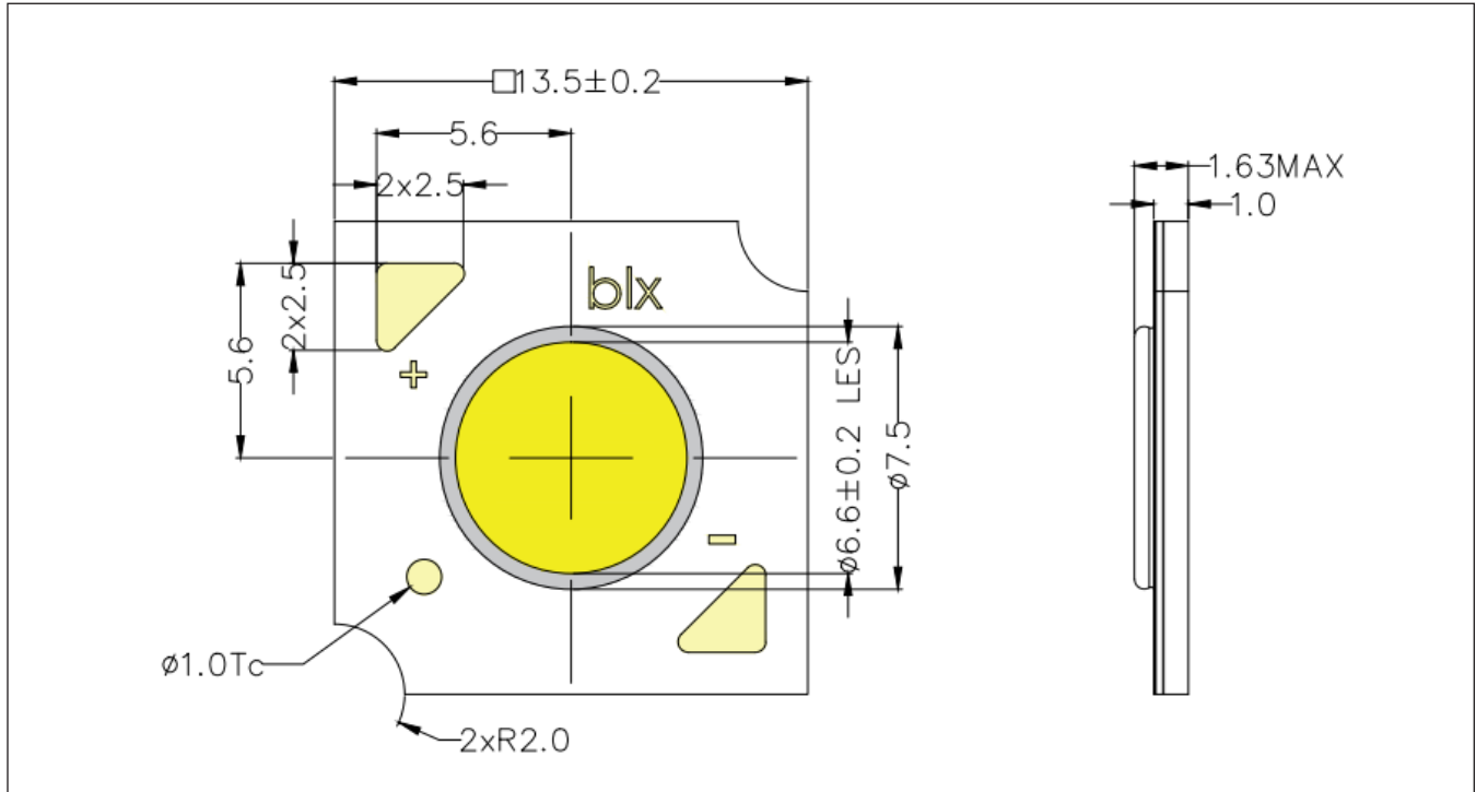
Figure 13: Drawing for V6 HD LED Array
