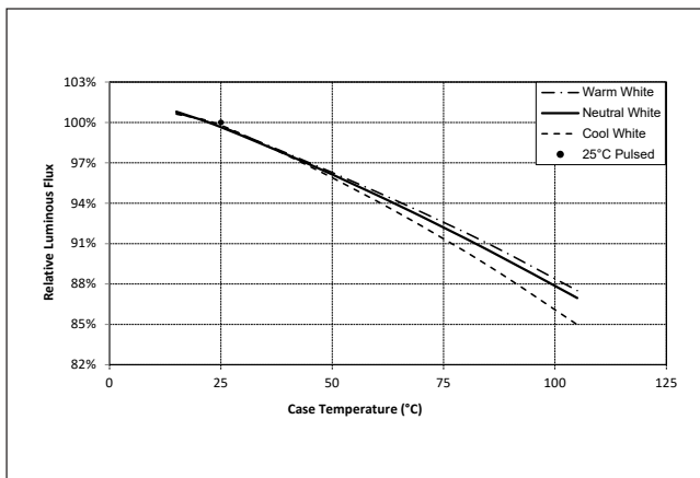
Figure 15: Typical DC Flux vs. Case Temperature
