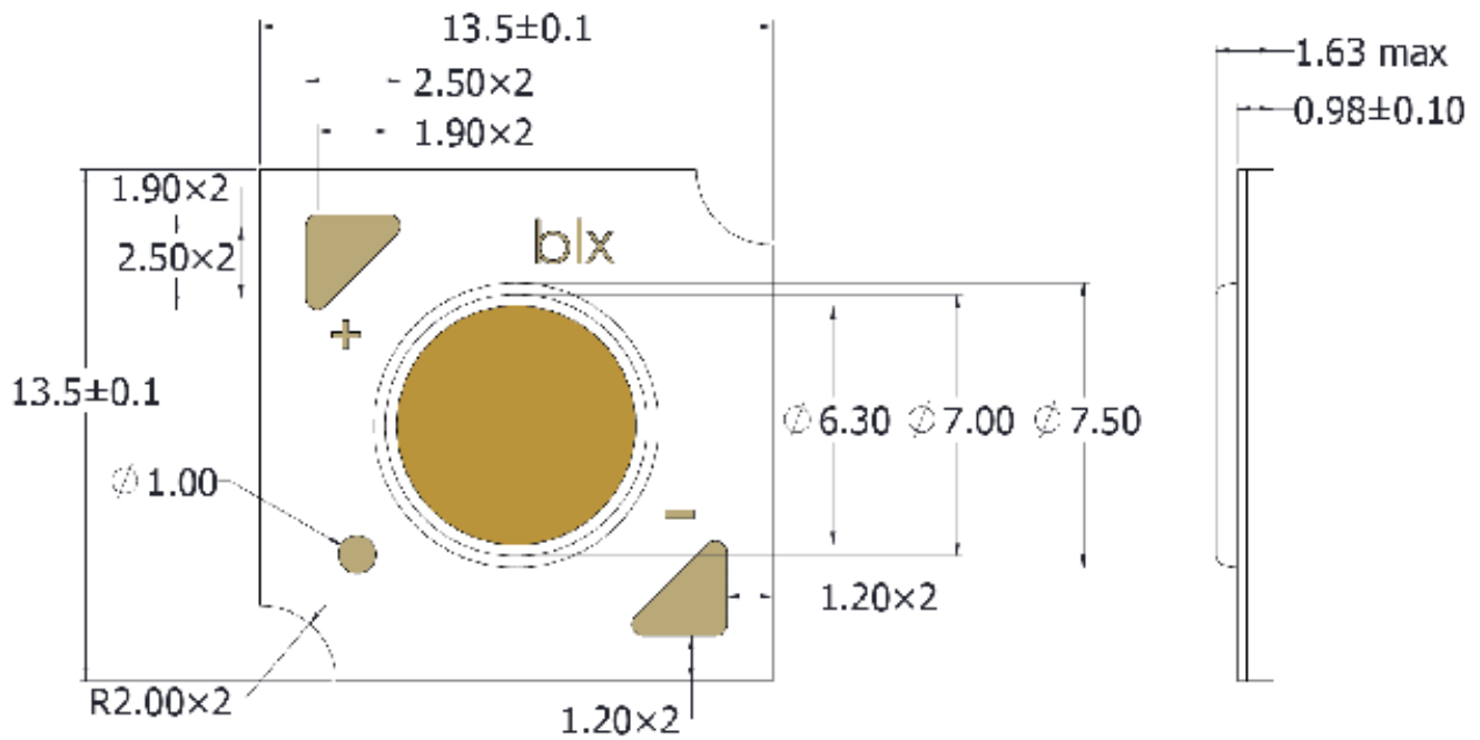
Figure 20: V6 HD LED Array
