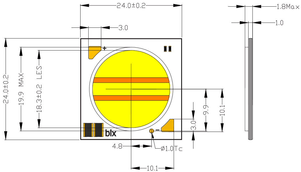
Figure 12: Mechanical Drawing
