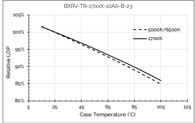
Figure 12: Relative Flux vs. Case Temperature
