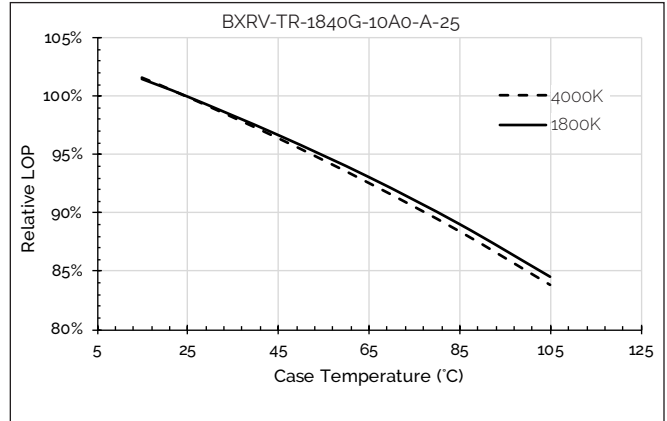
Figure 14: Relative Flux vs. Case Temperature
