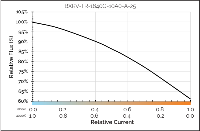
Figure 27: Relative Flux vs. Relative Current
