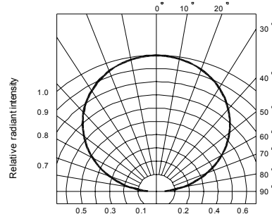
Fig.6 Radiation diagram
