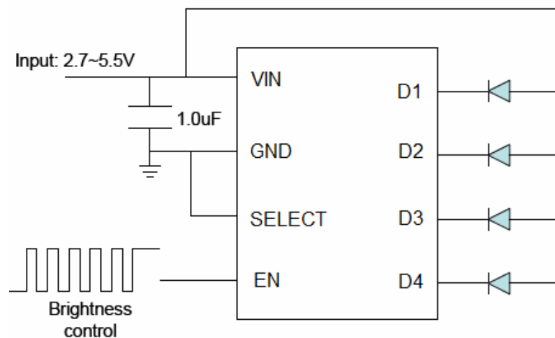
Figure 1: Application Circuit for Co-Anode Connection.
