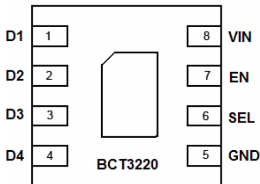
DFN2x2-8L Package
