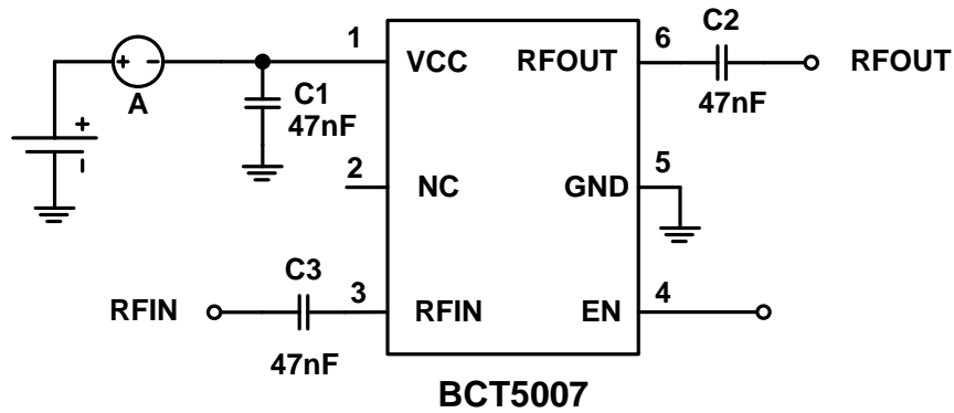
Figure 10. BCT5007 DC Test diagram
