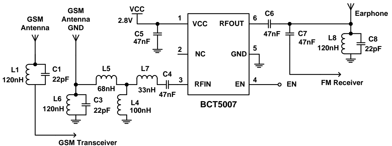
Figure 2. BCT5007 typical application circuit
