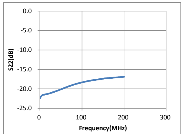
Figure 6. Output Return Loss(S22)
