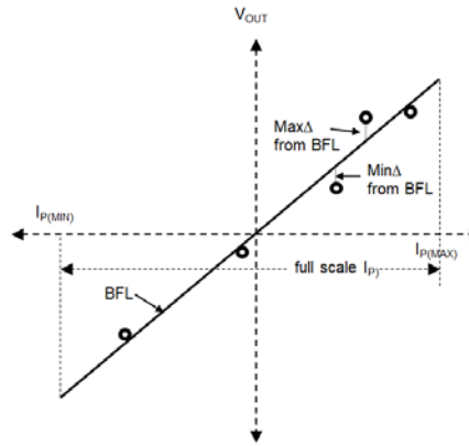
Figure 11: Nonlinearity Calculation
