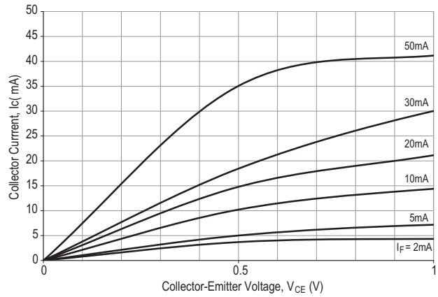
Figure 10 Collector Current vs. Small Collector-Emitter Voltage
