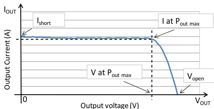
Figure 2: Illustration of a Typical I-V Curve of Optical Power Converters
