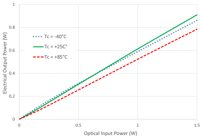
Figure 4: Typical Electrical Output Power vs. Optical Input Power of AFBR-POCx04L at Different Case Temperatures
