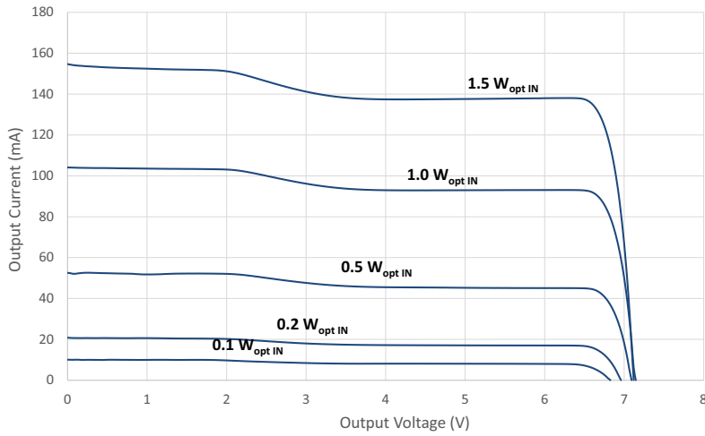
Figure 6: Typical I-V Curves (at T_C = +25^\circ\text{C} ) of AFBR-POCx06L at Different Optical Input Power
