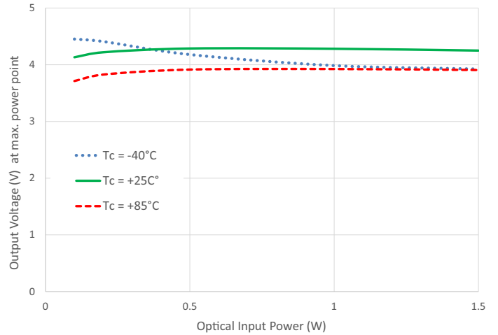
Figure 5: Typical Output Voltage vs. Optical Input Power of AFBR-POCx04L at Different Case Temperatures
