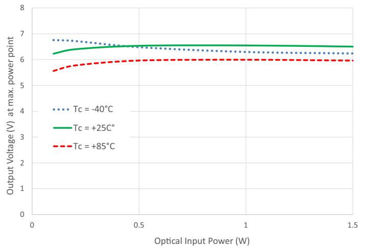
Figure 8: Typical Output Voltage vs. Optical Input Power of AFBR-POCx06L at Different Case Temperatures
