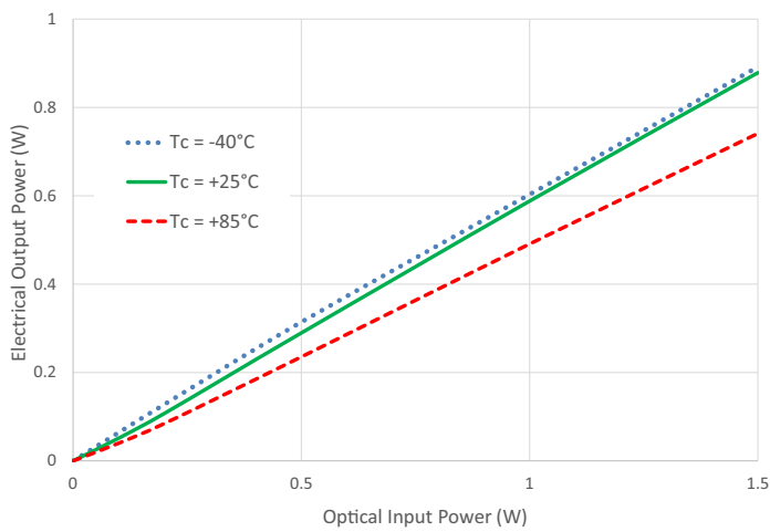
Figure 7: Typical Electrical Output Power vs. Optical Input Power of AFBR-POCx06L at Different Case Temperatures
