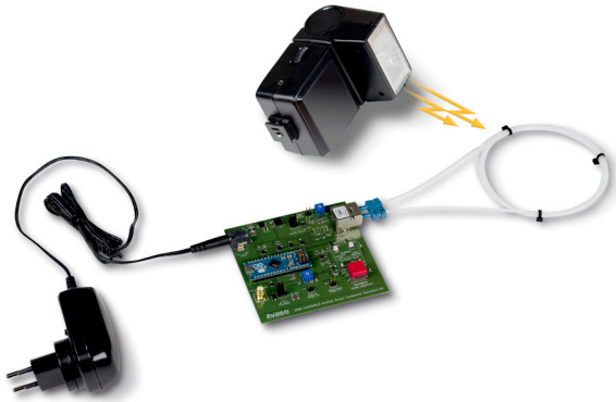
Figure 6. Configuration used to test the arc flash event detection alarm of the evaluation board
