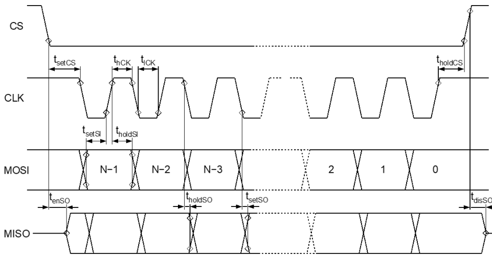
Figure 16: SPI Timing Diagram
