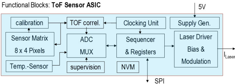
Figure 4: Functional Block Diagram of Sensor ASIC within AFBR-S50MV85G
