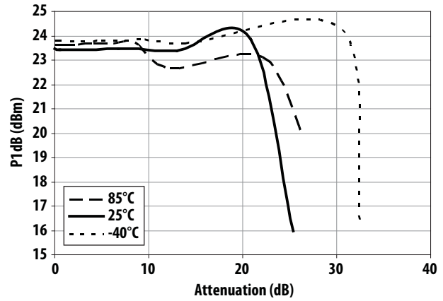
Figure 37. P1dB vs Attenuation and Temperature at 2500MHz
