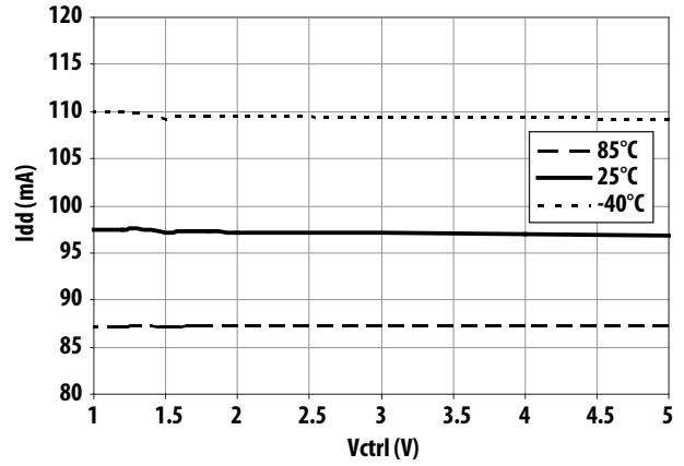
Figure 49. Current ( I_{dd} ) vs Control Voltage and Temperature
