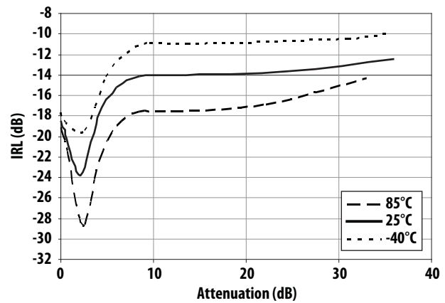
Figure 39. IRL vs Attenuation and Temperature at 2500MHz
