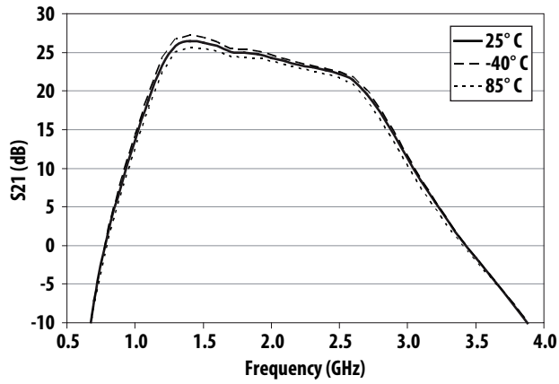
Figure 34. S21 vs Freq at 1960 MHz
