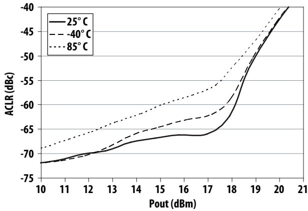
Figure 28. ACLR (Dual Carrier Signal) vs Pout at 1840 MHz
