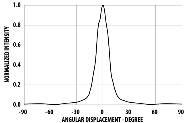
Figure 7 Radiation Pattern for X Axis -15°
