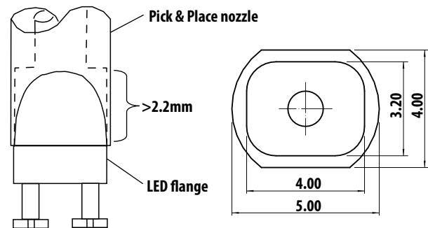
Figure 18 Nozzle Diagram
