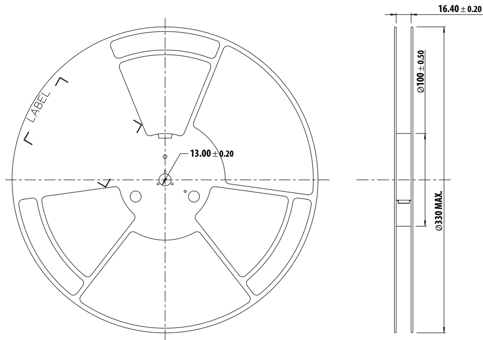
Figure 13 Reel Dimension
