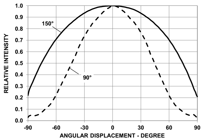
Figure 7: Radiation Pattern
