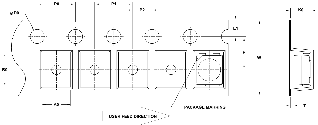
Figure 11: Carrier Tape Dimensions
