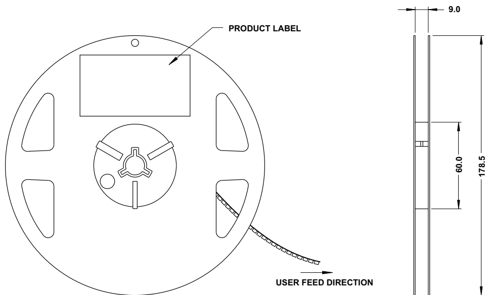
Figure 12: Reel Dimensions
