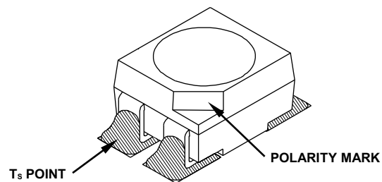
Figure 15: Solder Point Temperature on PCB
