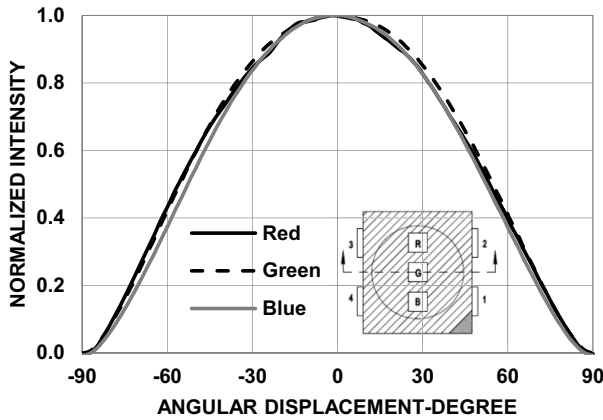
Figure 10: Radiation Pattern for X-axis
