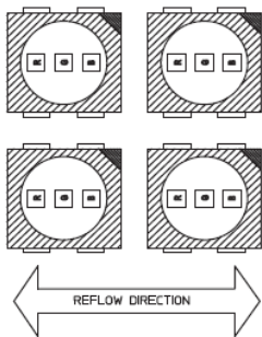
Figure 16: Recommended Board Reflow Direction
