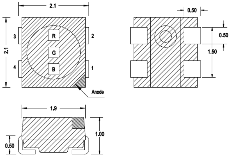
Figure 1: Package Drawing
