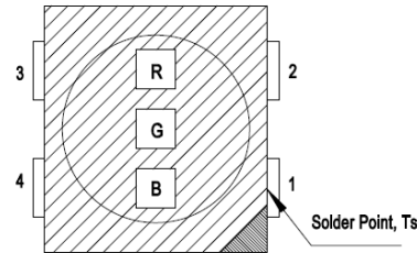
Figure 17: Solder Point Temperature on the PCB
