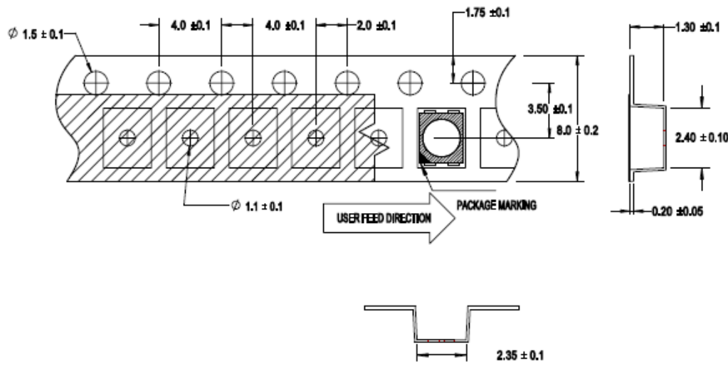
Figure 13: Carrier Tape Dimensions
