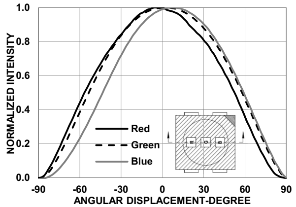
Figure 11: Radiation Pattern for Y-axis
