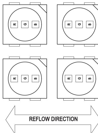
Figure 16: Recommended Board Reflow Direction
