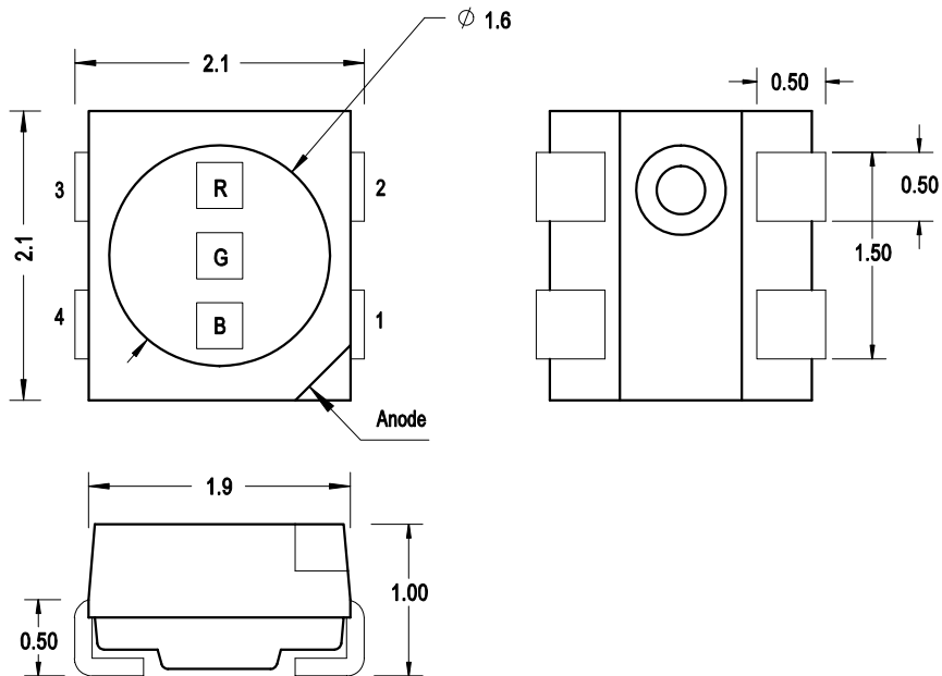
Figure 1: Package Drawing
