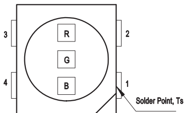
Figure 17: Solder Point Temperature on PCB
