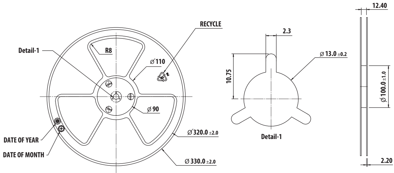
Figure 17 Reel Dimensions
