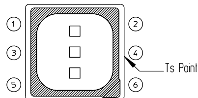
Figure 17: Solder Point Temperature on PCB
