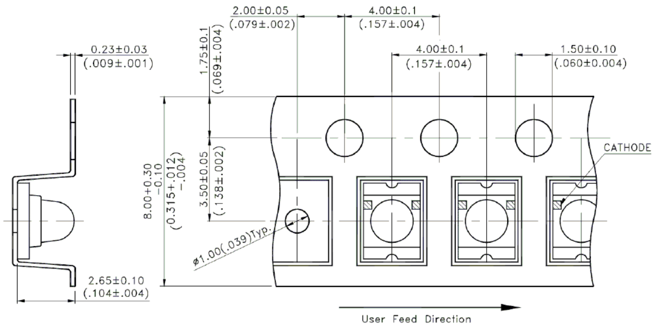
Figure 11: Tape Dimensions
