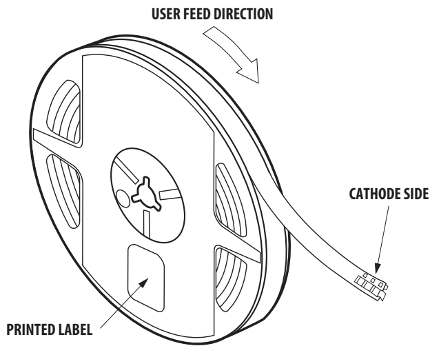
Figure 9: Reeling Orientation
