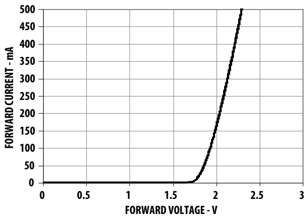
Figure 7 Forward Current vs. Forward Voltage
