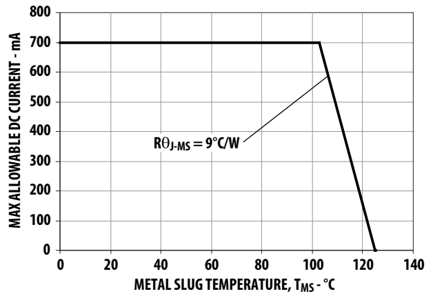
Figure 11. Maximum Forward Current vs. Ambient Temperature. Derated based on T JMAX = 125°C, R θMS = 9°C/W.
