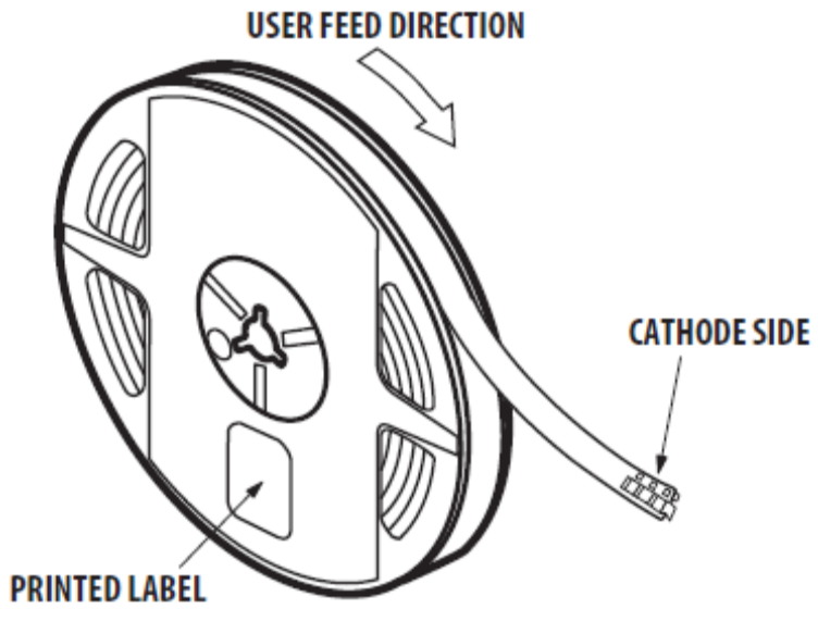
Figure 16. Reeling Orientation
