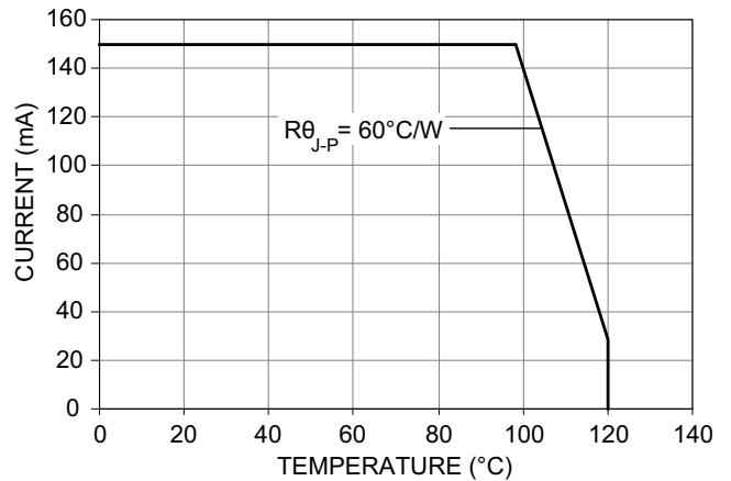
Figure 7: Max. Forward Current vs. Solder Point Temperature Derated Based on T_{JMAX} = 125^{\circ}C , R_{\theta J-P} = 60^{\circ}C/W .
