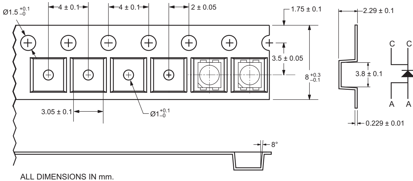
Figure 16: Tape Dimensions
