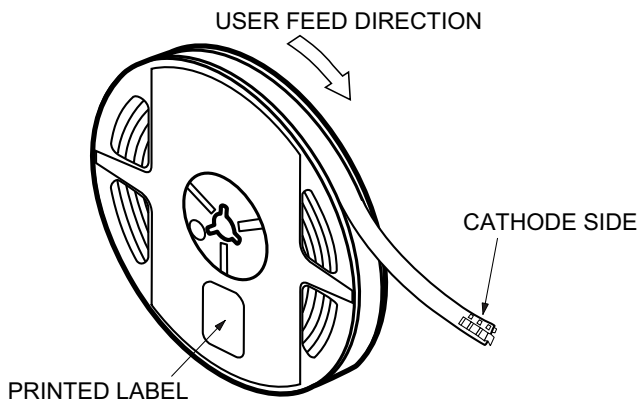
Figure 17: Reeling Orientation
