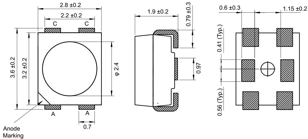
Figure 1: Package Drawing
