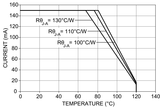
Figure 6: Max. Forward Current vs. Ambient Temperature Derated Based on T_{JMAX} = 125^{\circ}C , R_{\theta J-A} = 130^{\circ}C/W , 110^{\circ}C/W , and 100^{\circ}C/W .
