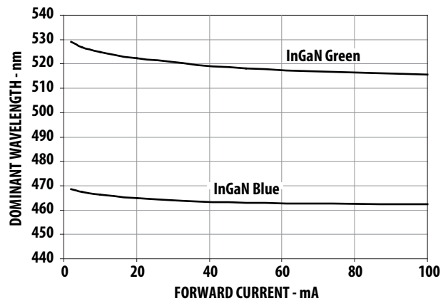
Figure 7: Dominant Wavelength Shift vs. Forward Current
